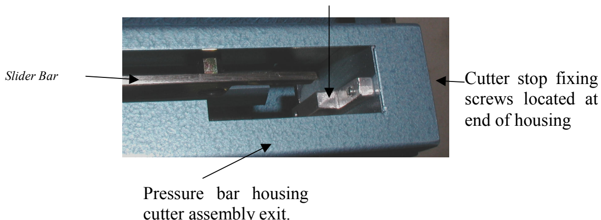
Aluminium Cutter Stop
