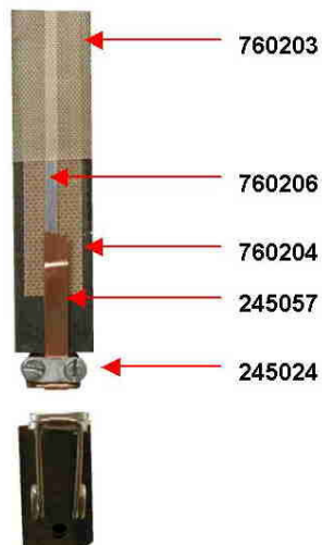
760211 – STD HEATER BAR ASSEMBLY
