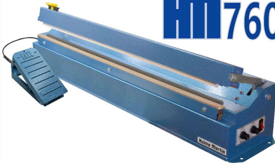
(Foot Operated, Large Capacity Impulse Heat Sealer) – Part No. 76002181
